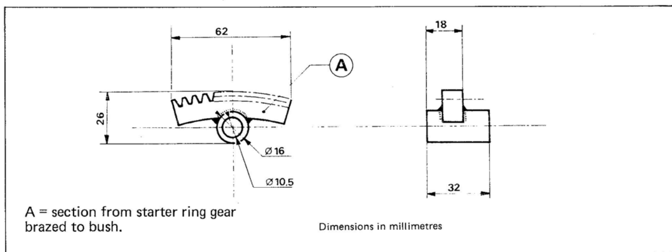
Starter ring gear locking tool
